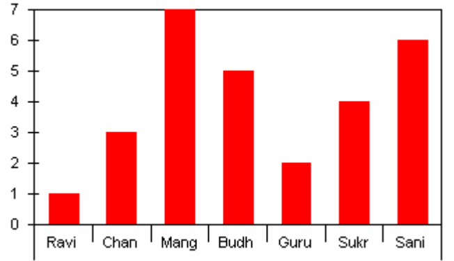
Planetary Longitudes
