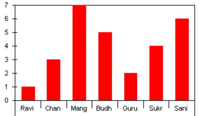
Planetary Longitudes
